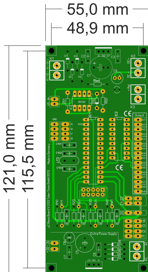
TT-Midi ChannelSwitcher Board Layout Version 2.0.3
